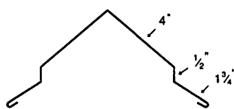
RIDGE CAP
