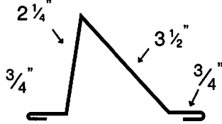
SNOW STOP
