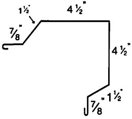
TRANSITION
