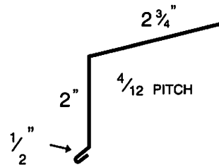
EAVE
