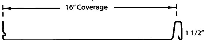
Snap Lock
