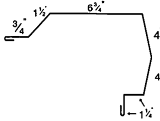
END WALL
